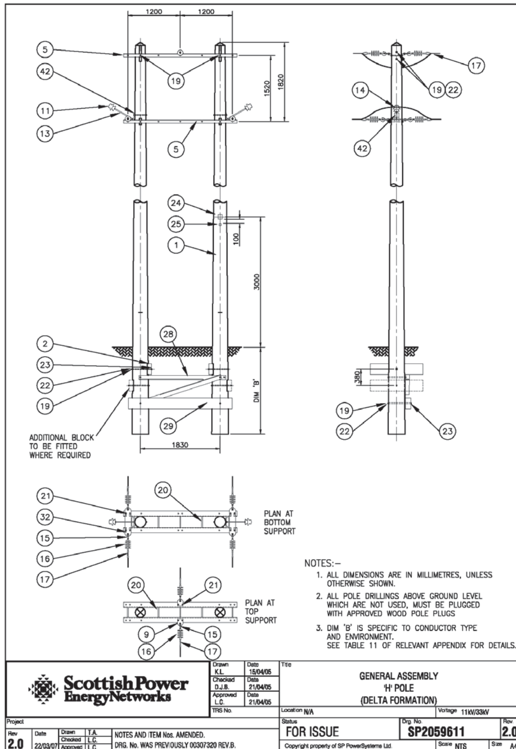
Figure 15 Delta “H” Pole Section or Section Angle (Drawing SP2059611)
